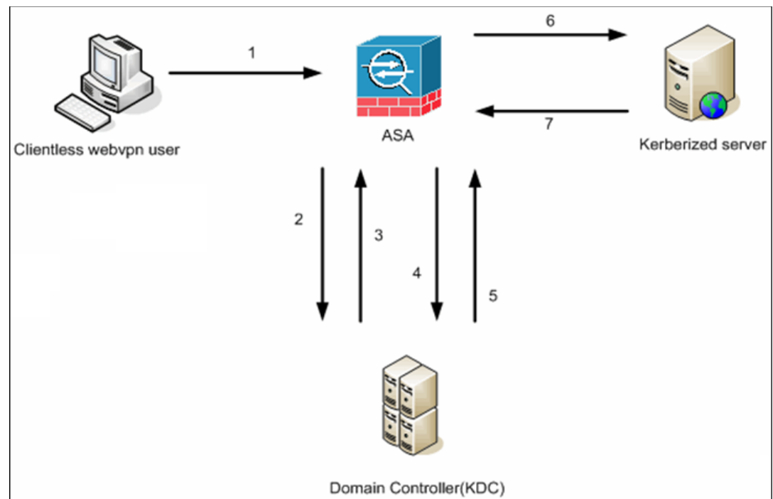
Figure 14-1 KCD Process
