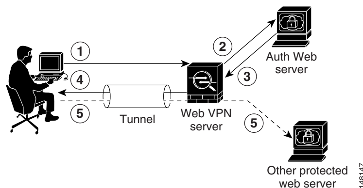
Figure 17-1 SSO Authentication Using HTTP Forms
