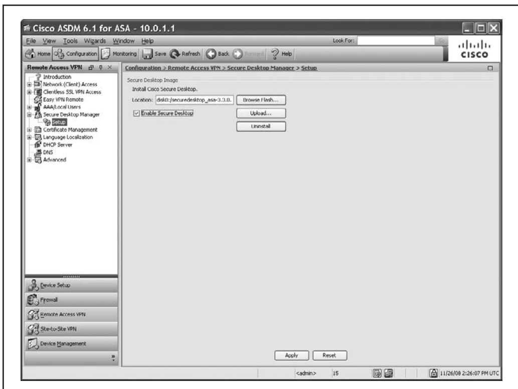
Figure 27-23. Installing CSD
