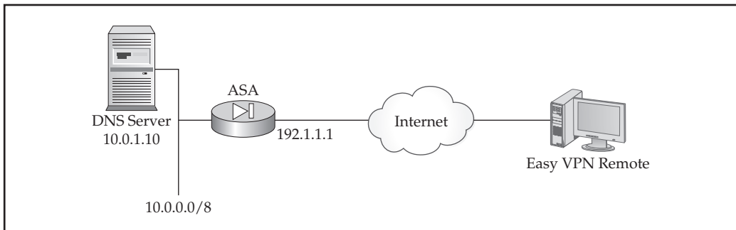
Figure 17-2. Easy VPN server example
