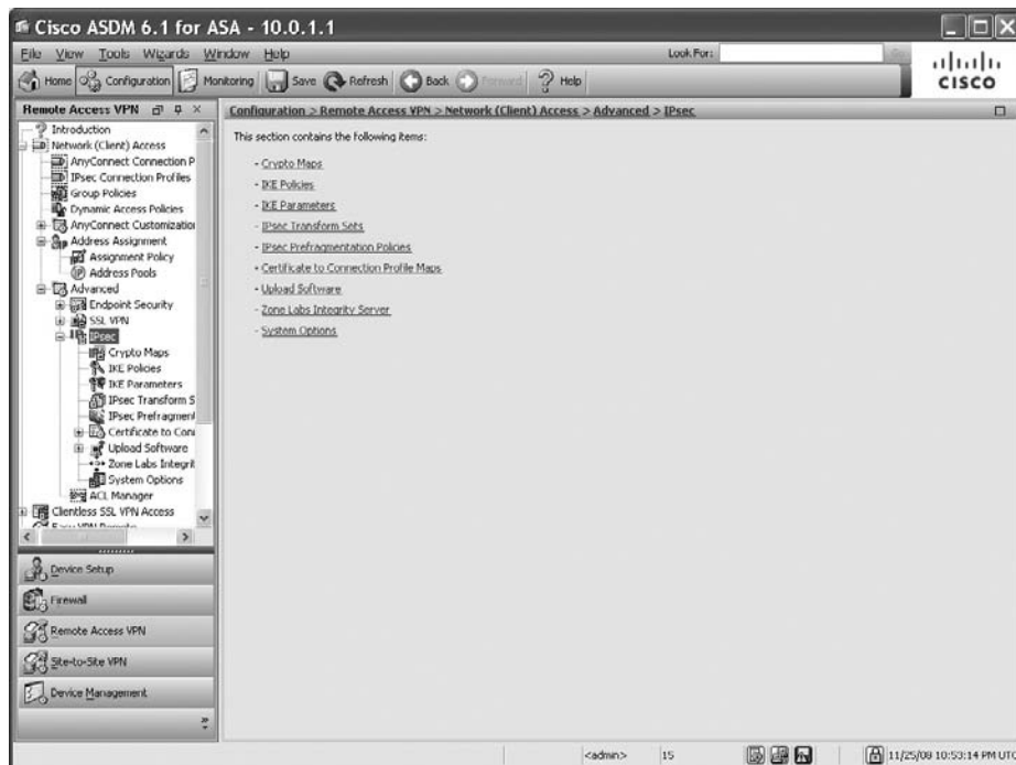
Figure 27-17. General Easy VPN IPsec properties
