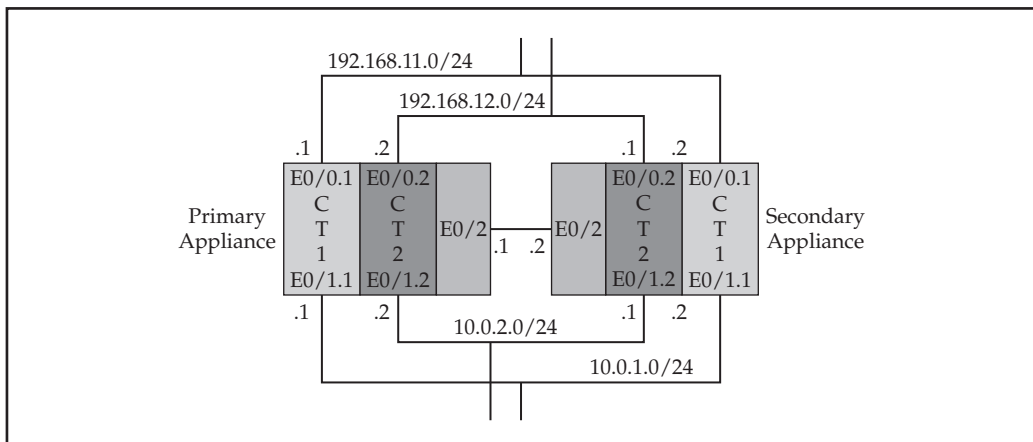
Figure 23-7. Active/active example using LBF
