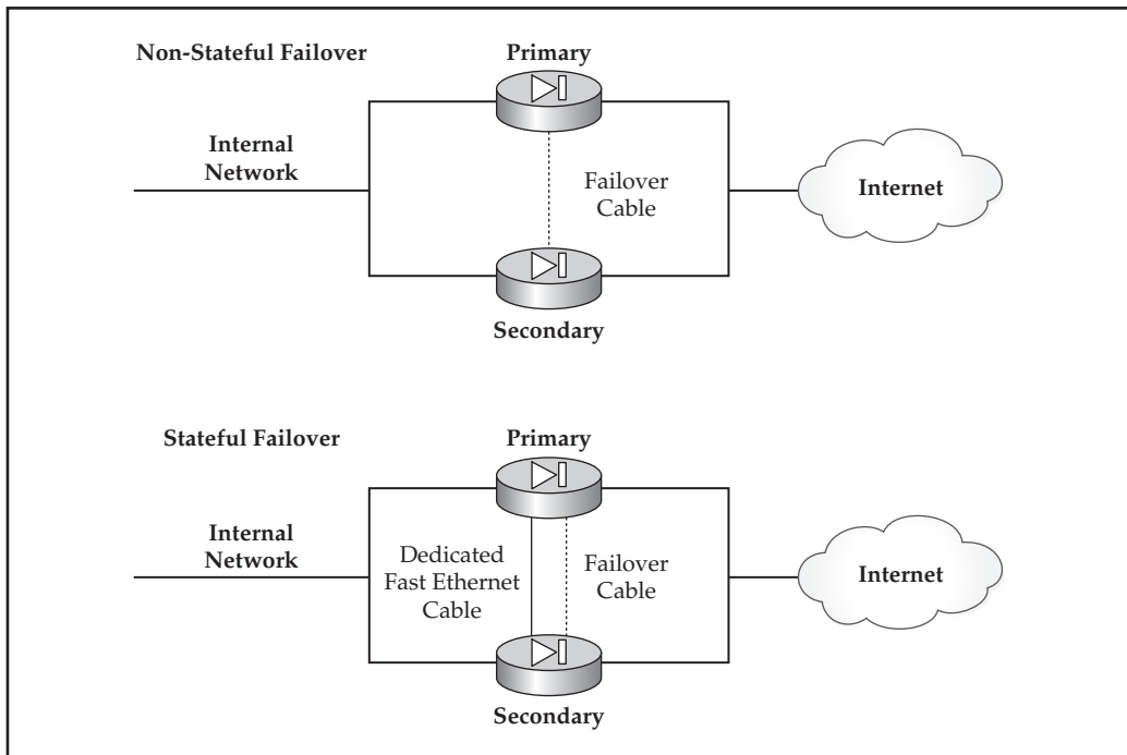
Figure 1-6. Hardware vs. stateful failover
