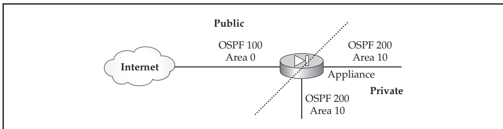
Figure 4-4. ASBR appliance performing redistribution
