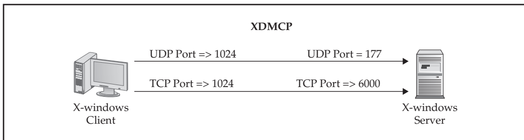
Figure 11-1. This is how an XDMCP session is established.
