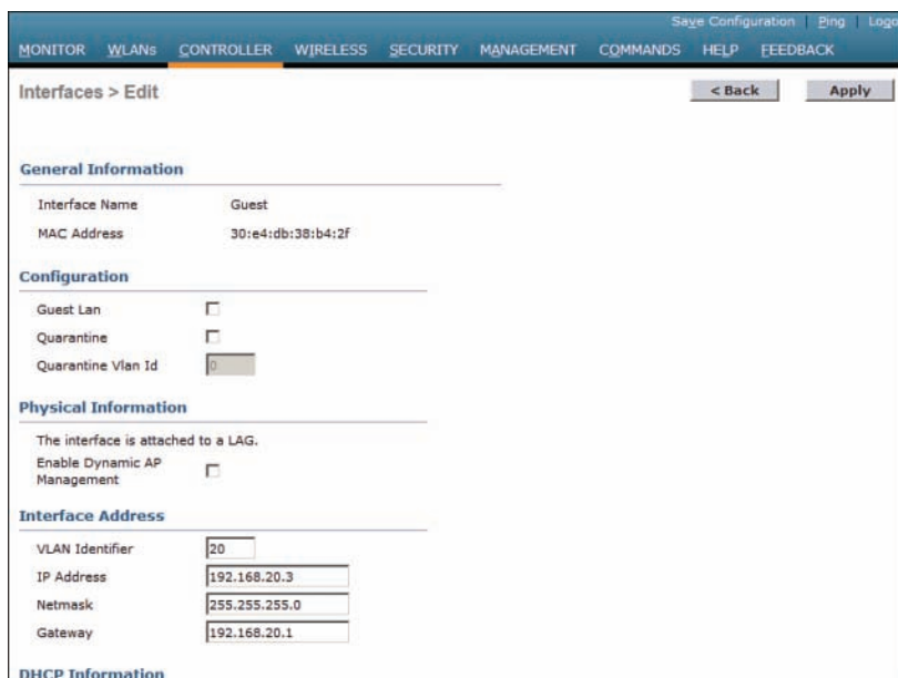
Figure 16-5 Configuring IP Address Information on the Guest Interface
