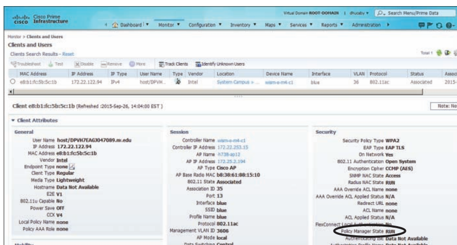
Figure 20-4 Displaying Client Details in PI
