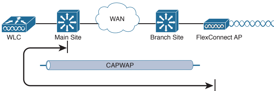
Figure 8-17 Split-MAC Architecture at a Branch Site
