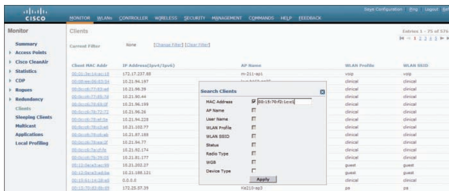
Figure 20-13 Displaying and Filtering Client Status Information on a Controller
