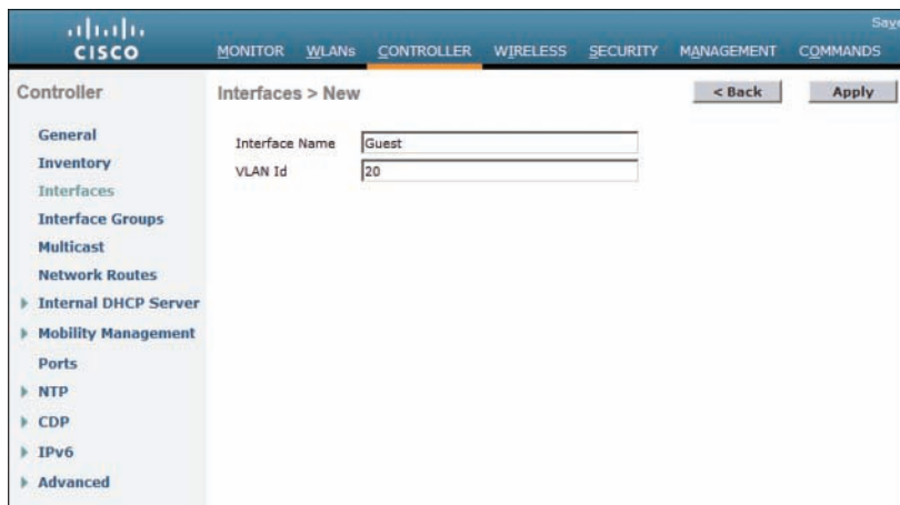
Figure 16-4 Creating a Controller Interface for a Guest WLAN
