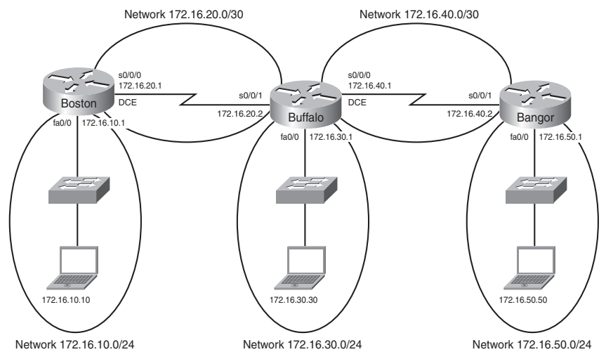
Figure 7-6 Network Topology for Static Route Configuration
