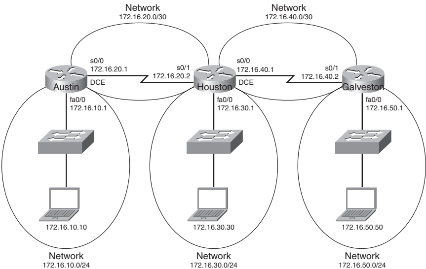
Figure 10-9 Network Topology for Single Area OSPF Configuration
