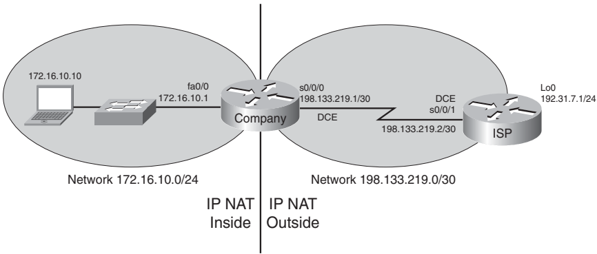
Figure 23-3 Port Address Translation Configuration
