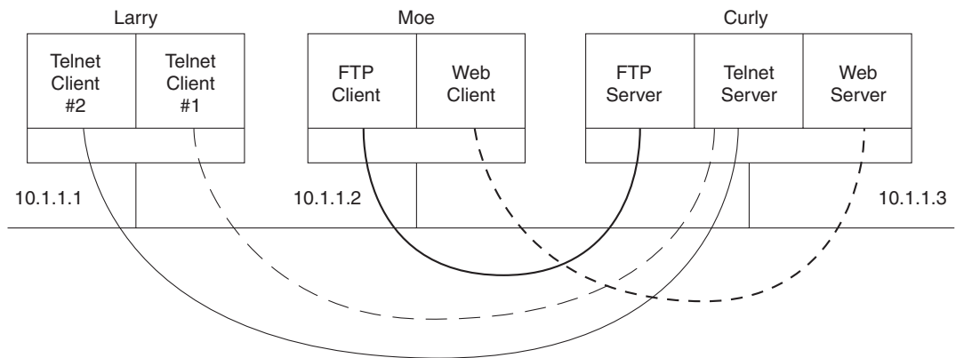
Figure 5-3 Connections Between Sockets
