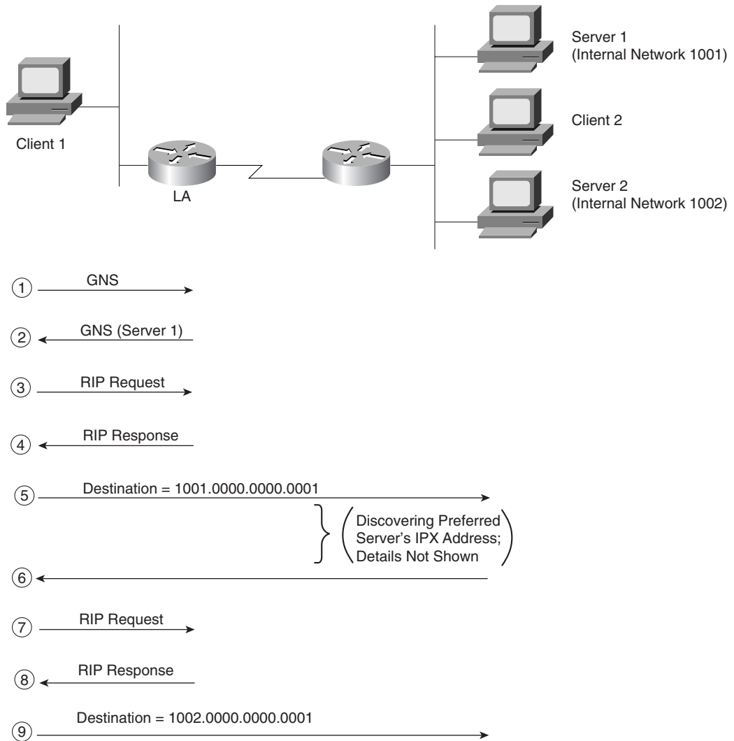
Figure 6-14 Client Initialization Flows
