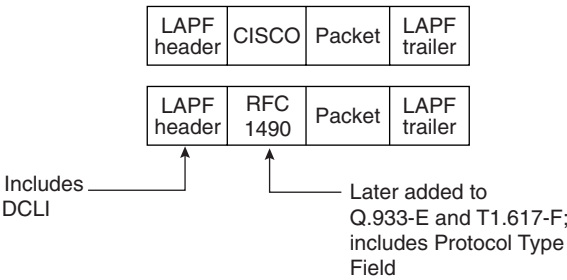
Figure 8-37 Cisco and RFC 1490/2427 Encapsulations
