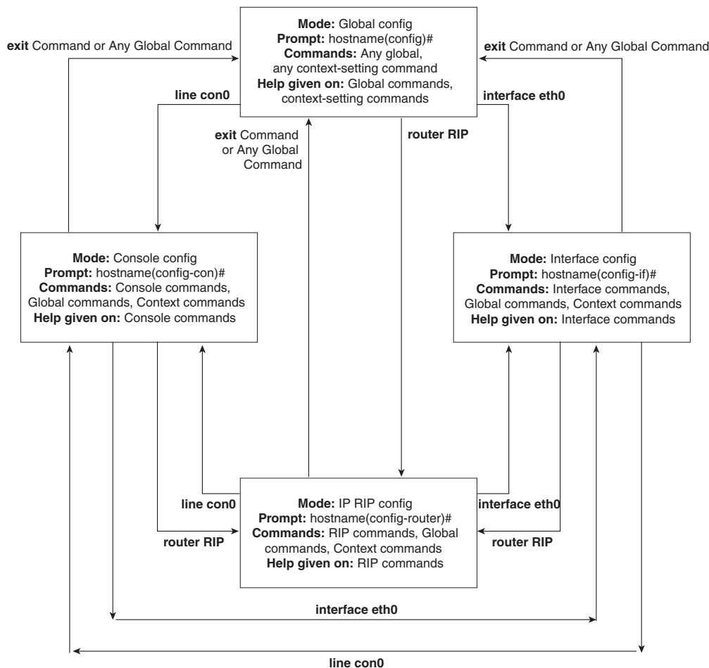
Figure 2-7 Relationships Among Context-Setting Commands
