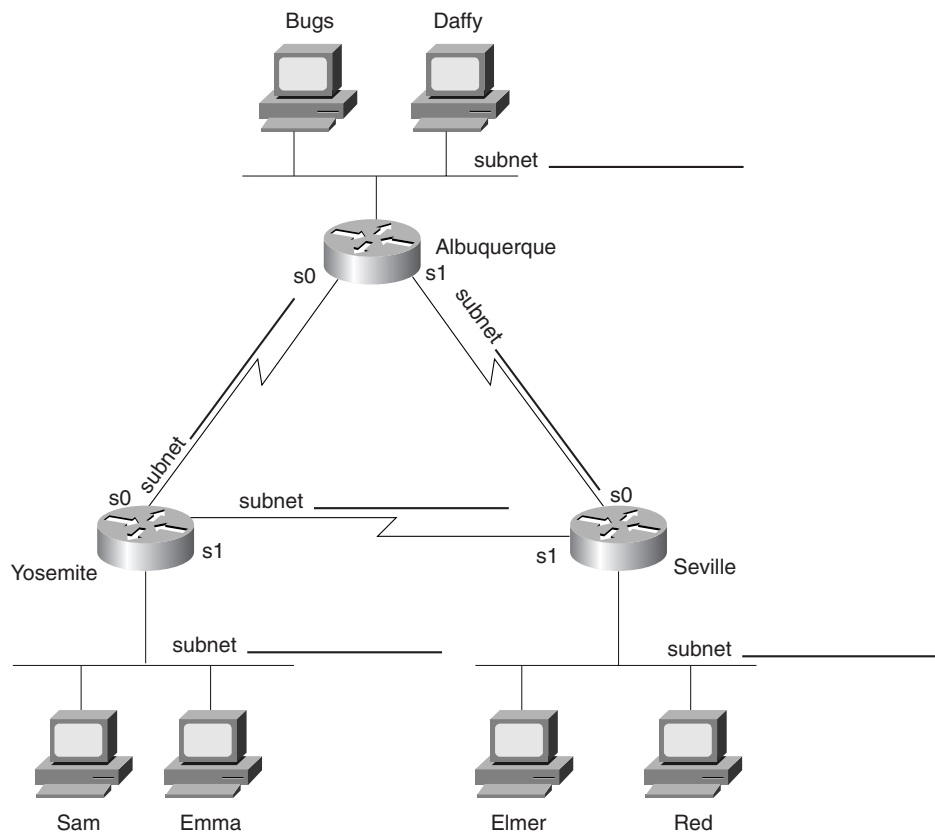
Figure 6-23 Scenario 6-1 Network Diagram
