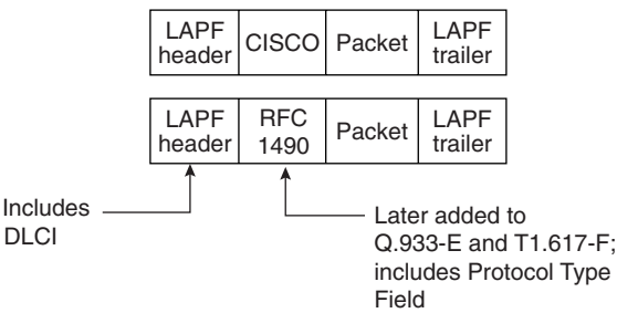
Figure 8-6 Cisco and RFC 1490/2427 Encapsulations
