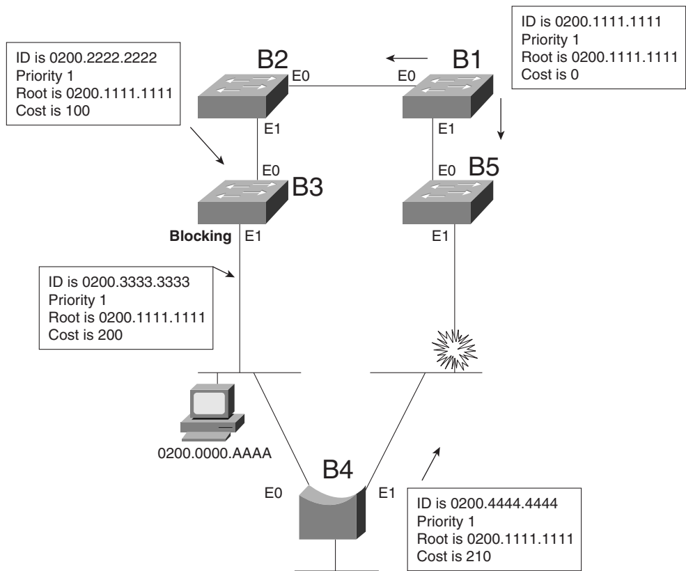
Figure 4-20 CBPDUs After Bridge 4's MaxAge Expires
