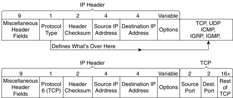
Figure 7-4 Extended Access List Matching Options
