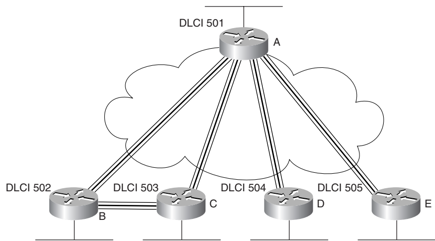
Figure 8-13 Hybrid of Full and Partial Mesh
