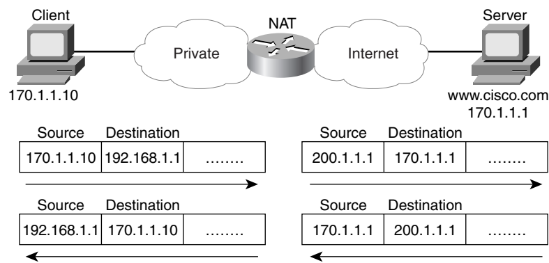
Figure 5-26 NAT IP Address Swapping—Unregistered Networks
