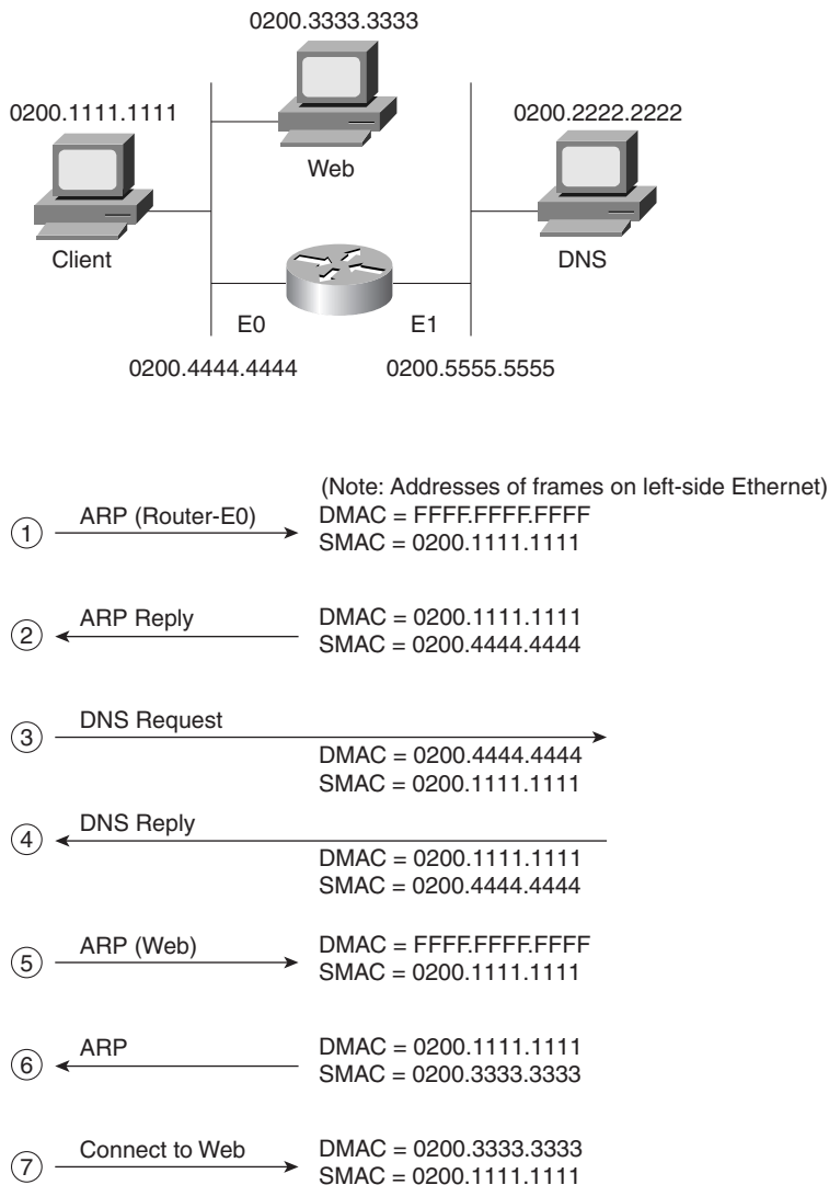
Figure 4-13 Example Protocol Flows—Using a Router
