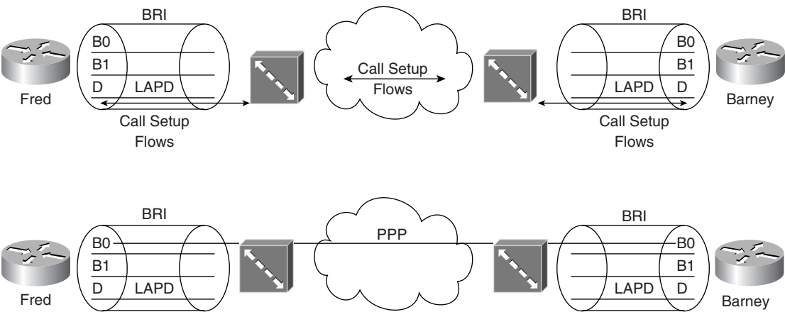
Figure 8-38 LAPD and PPP on D and B Channels
