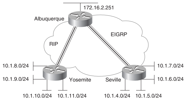
Figure 6-13 Network Environment for Use with show ip route Options
