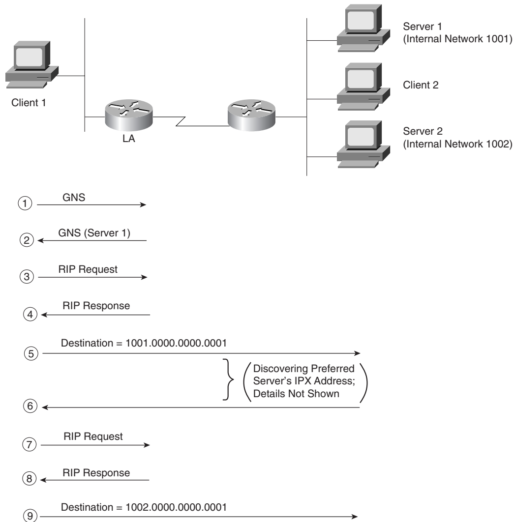
Figure 6-22 Client Initialization Flows
