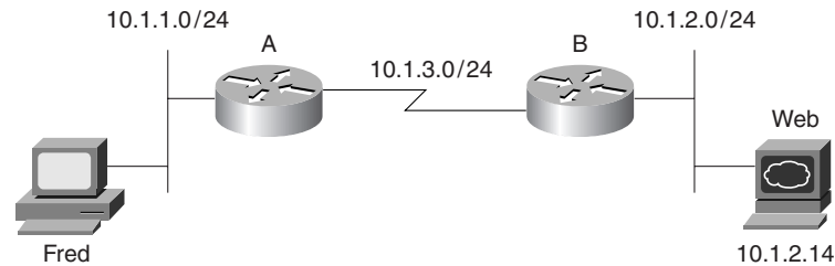
Figure 5-13 Sample Network for Discussing ICMP Unreachable
