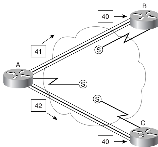
Figure 8-8 Frame Relay Local Addressing, with Different DLCIs on Each End
