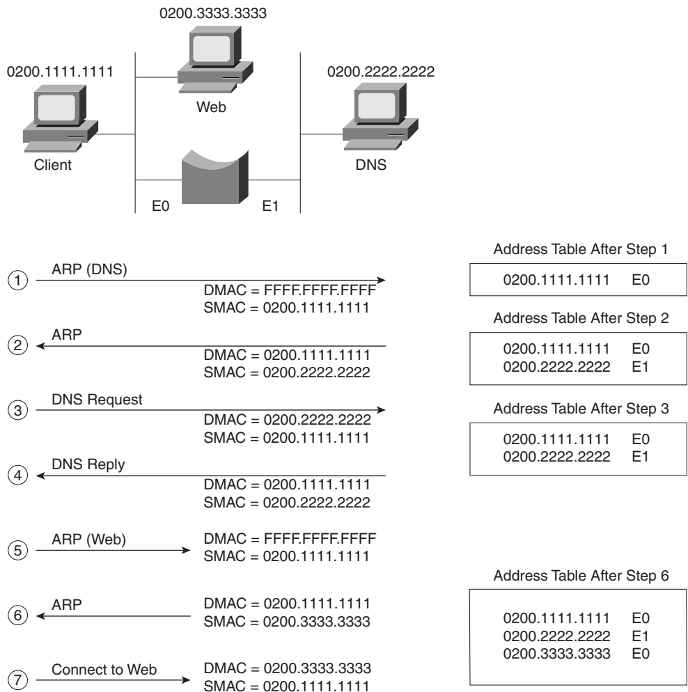
Figure 4-7 Example Protocol Flows—Using a Transparent Bridge
