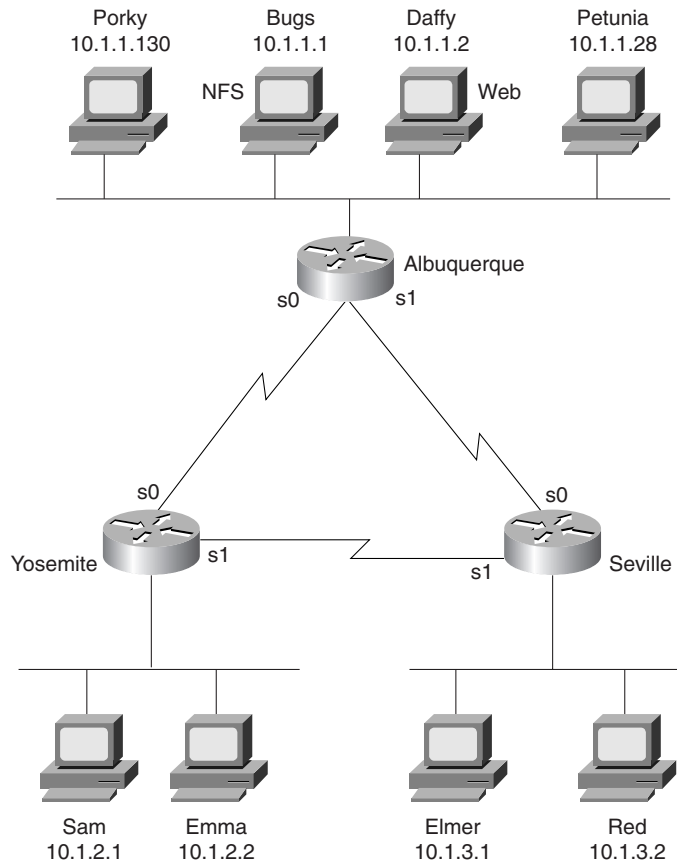
Figure 7-5 Network Diagram for Extended Access List, Example 2
