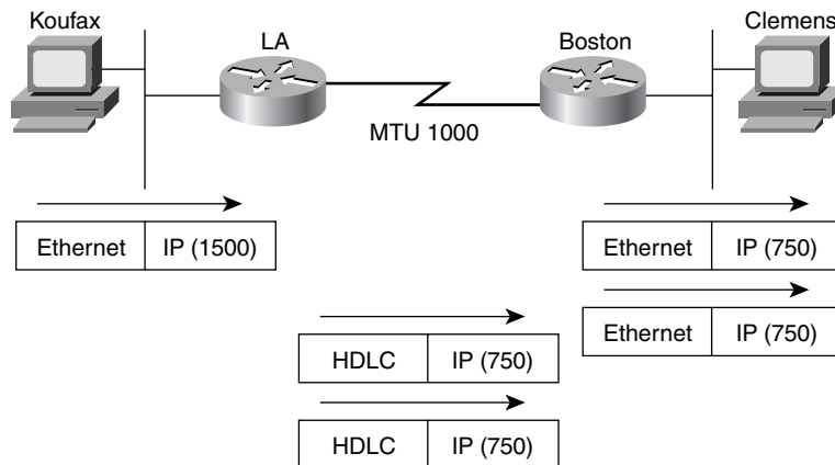
Figure 5-29 IP Fragmentation
