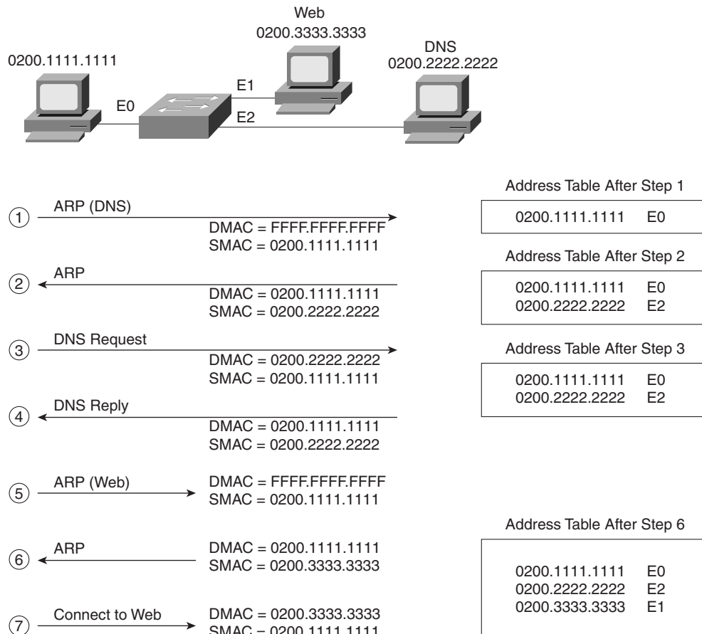
Figure 4-8 Example Protocol Flows—Using a Switch
