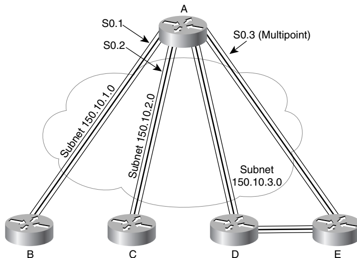
Figure 5-28 Frame Relay Subnets with Point-to-Point and Multipoint Subinterfaces
